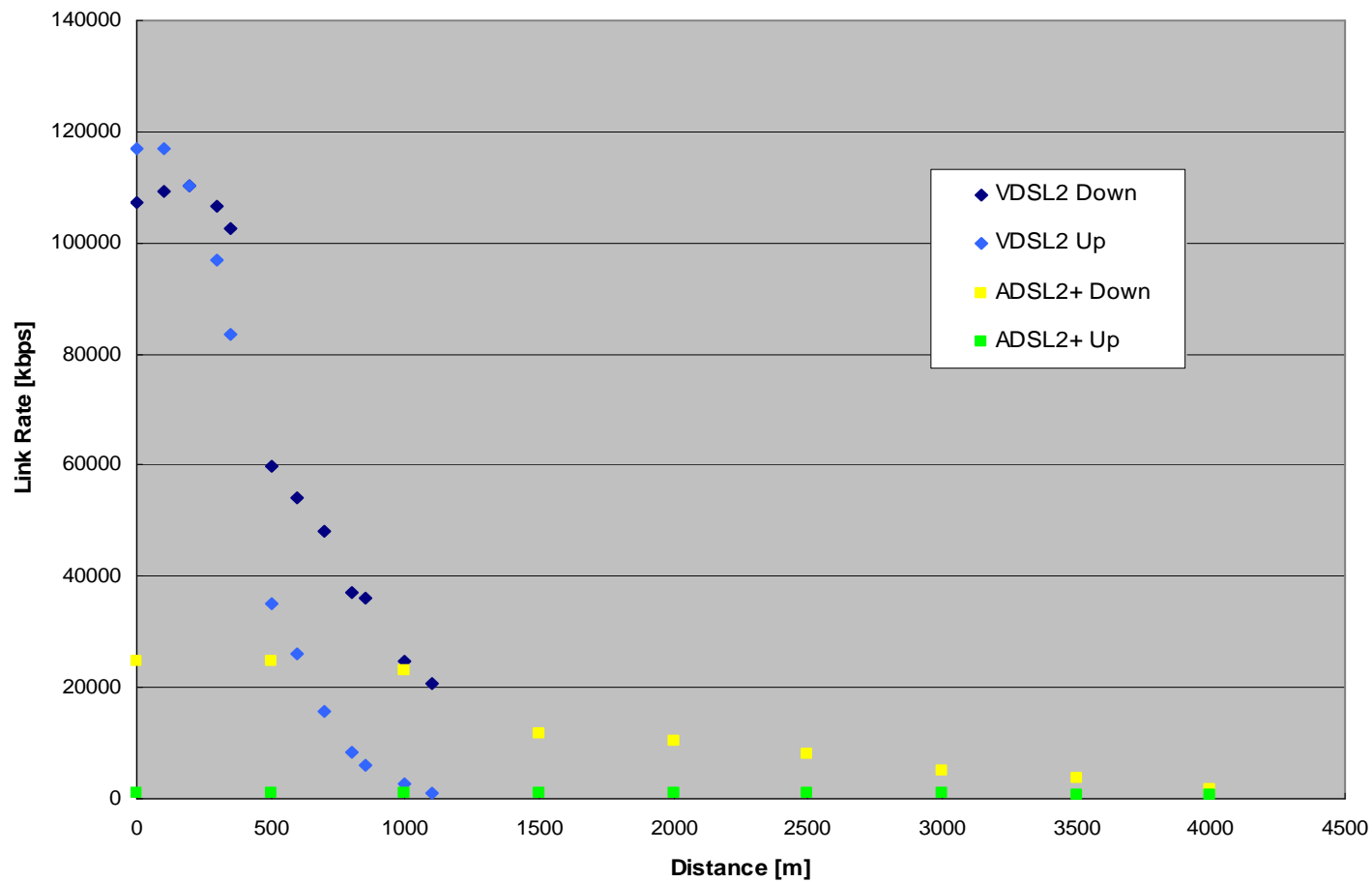
HP2-160 VDSL2 & ADSL2+ Performance
