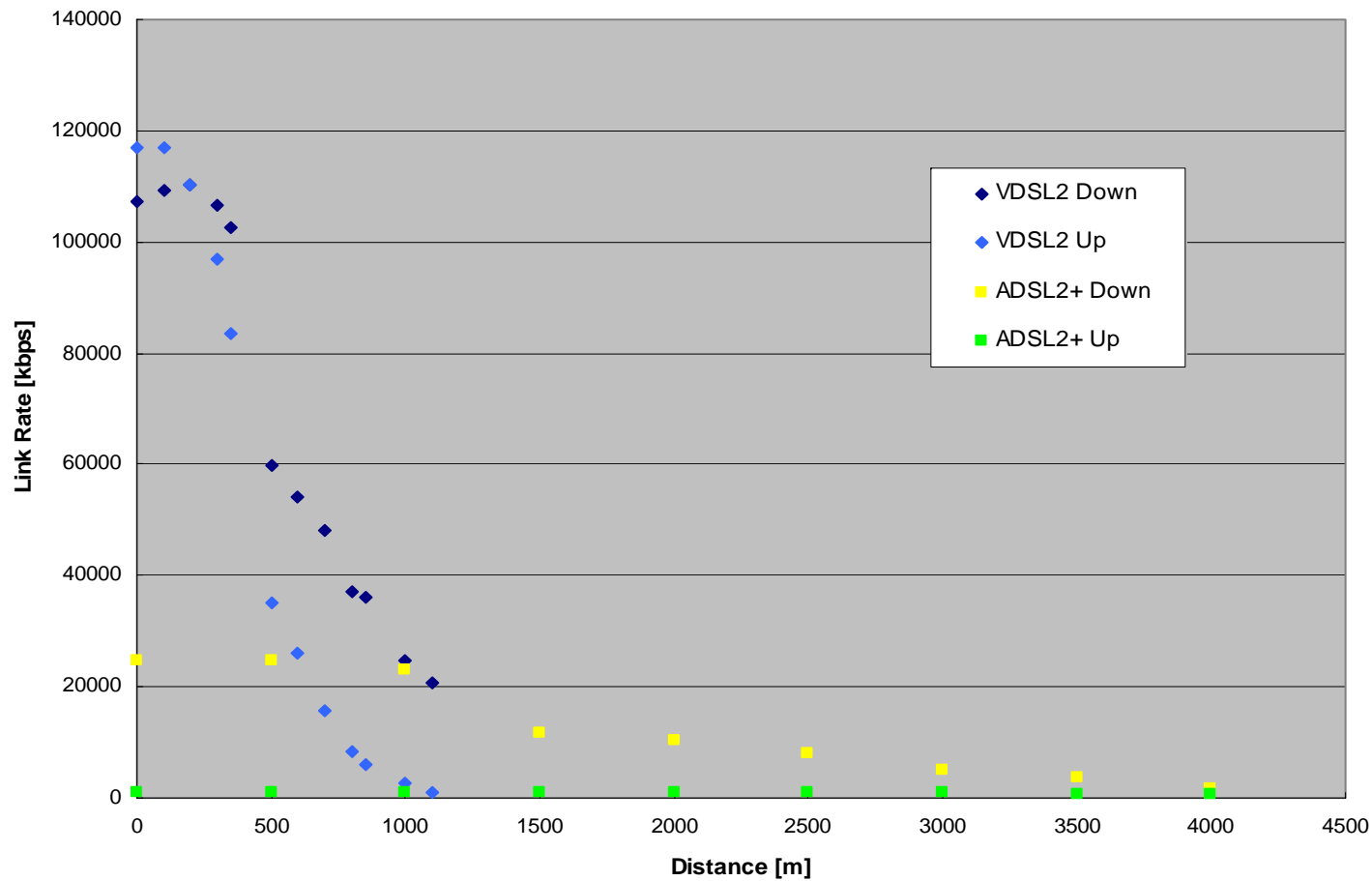
HP-160 VDSL2 & ADSL2+ Performance
